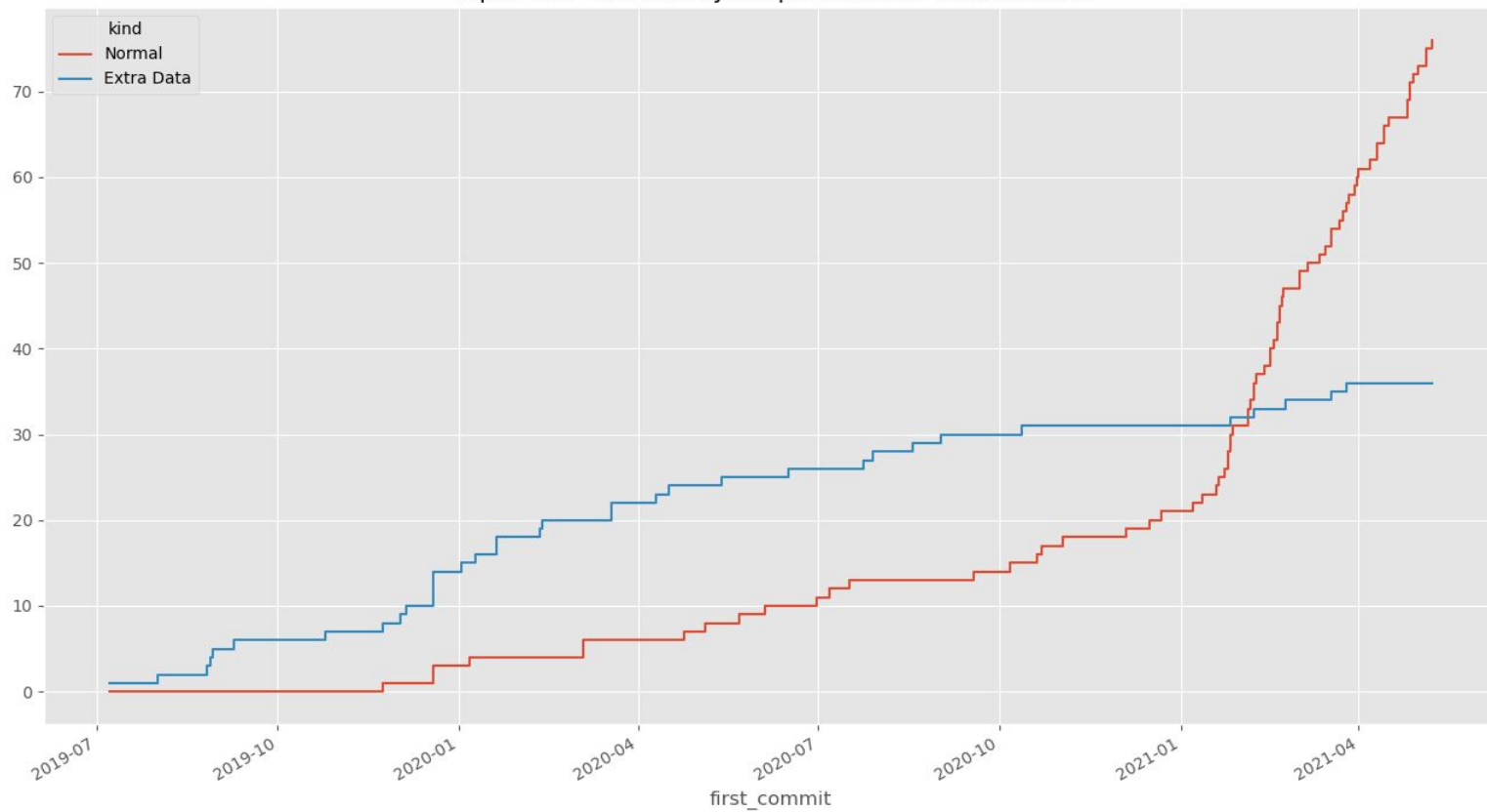
Repos with Commits by Flatpak External Data Checker
